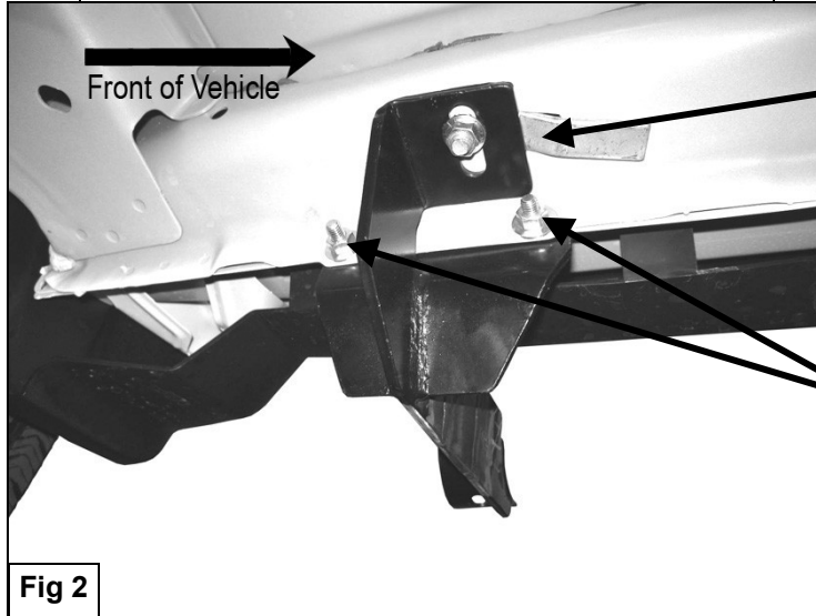
Driver Side Rear Mounting Bracket Shown
