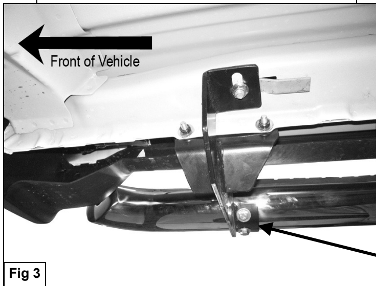
Passenger Side Front Mounting Bracket Shown
