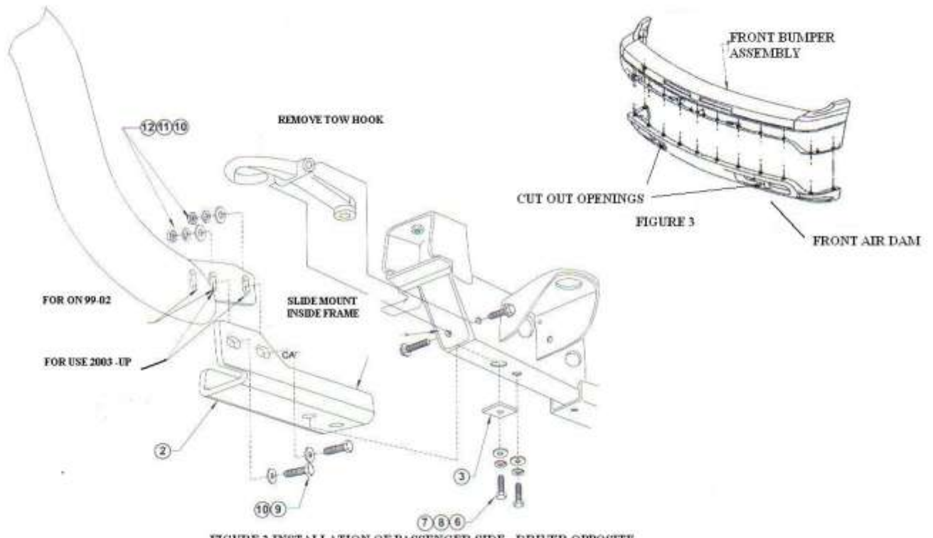
FIGURE 2 INSTALLATION OF PASSENGER SIDE- DRIVER OPPOSITE
