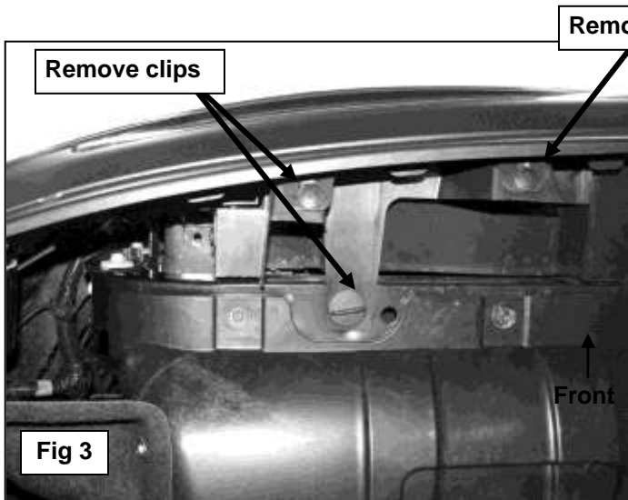
Remove splash guard (passenger side pictured from below)
